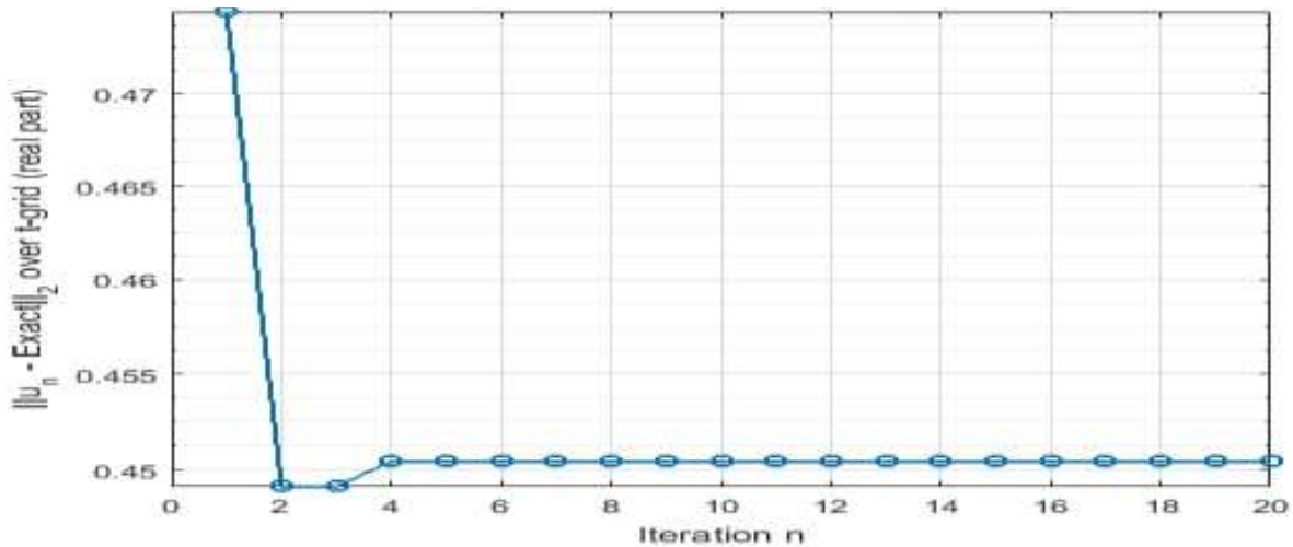
Figure 4. AVIM Convergence for Schrödinger Equation
