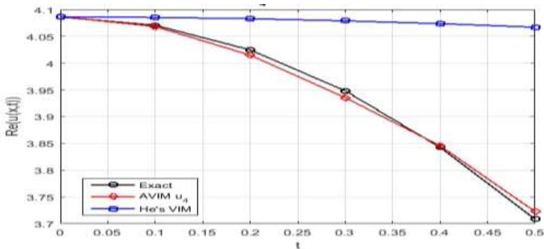
Figure 3. AVIM applied to the Schrödinger Equation
