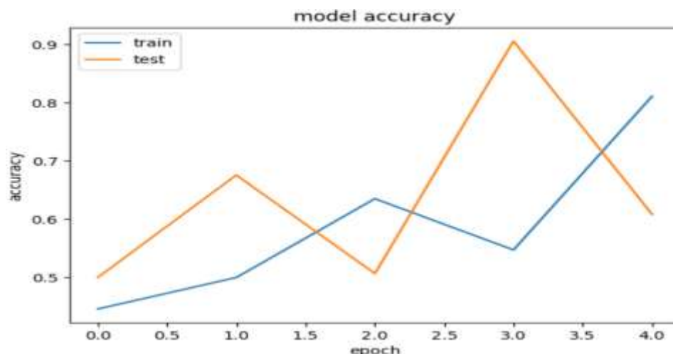
Figure 12. Training and Validation Accuracy of CNN Model Over Epochs.
